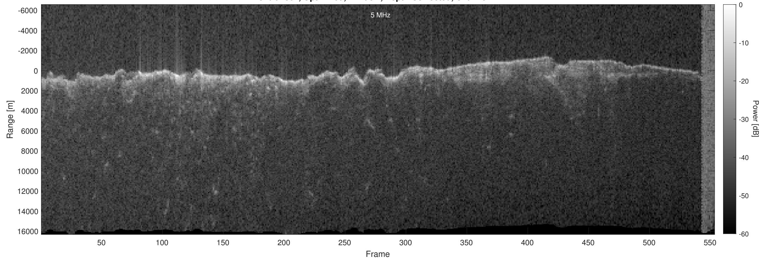
Orbit 4501, Optimized, Window, Depth-Corrected, Channel 2
