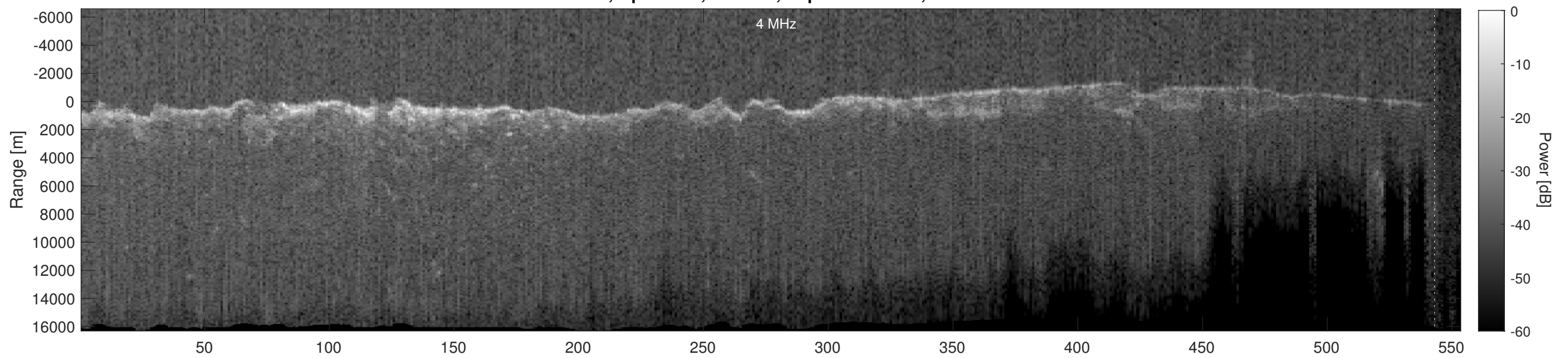
Orbit 4501, Depth-Corrected Cluttergram
