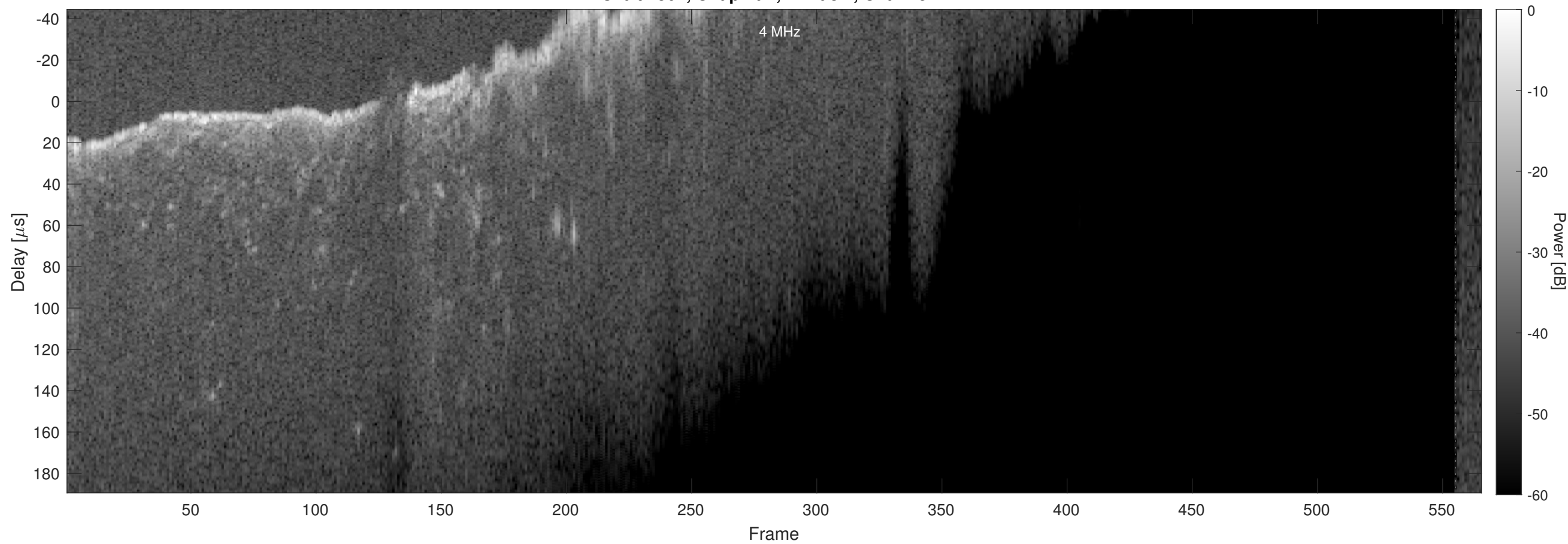
Orbit 4504, Chapman, Window, Channel 2
