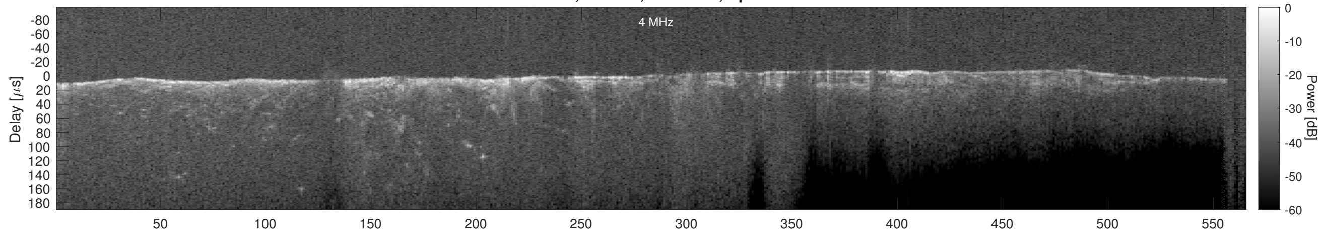
Orbit 4504, Cluttergram
