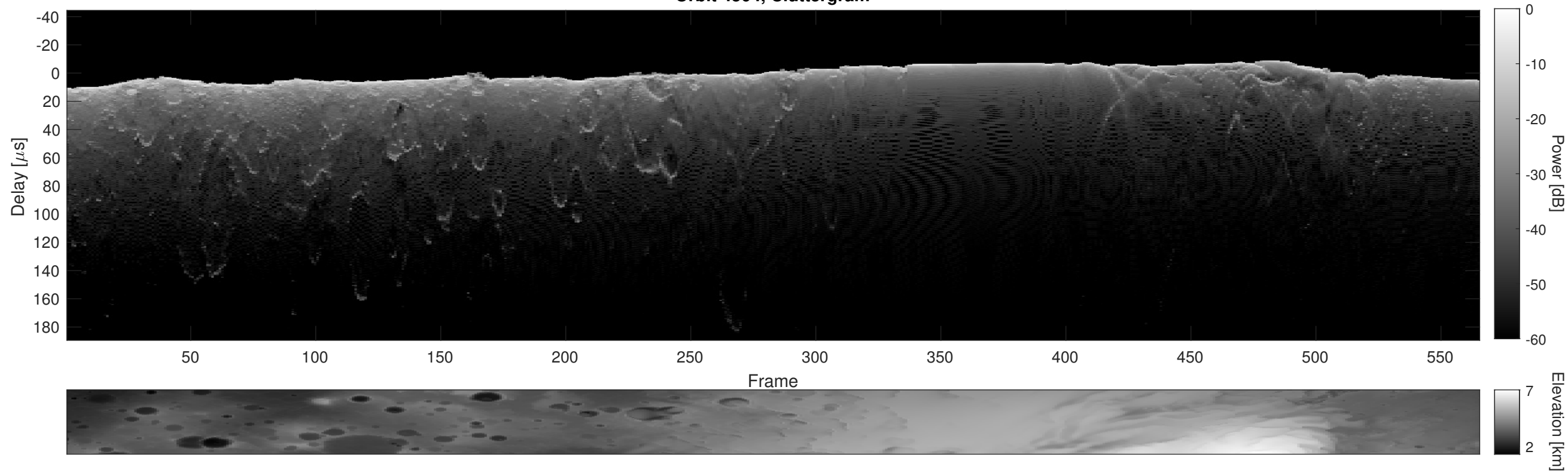
Orbit 4504, Cluttergram
