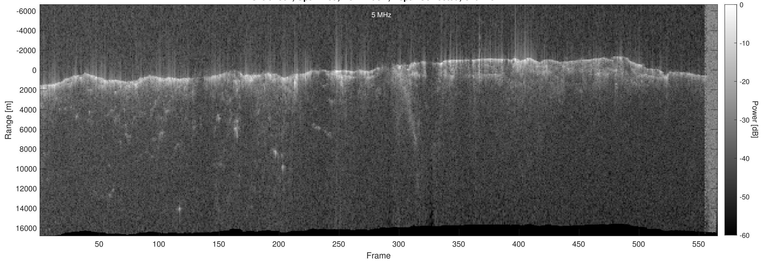
Orbit 4504, Optimized, No Window, Depth-Corrected, Channel 2
