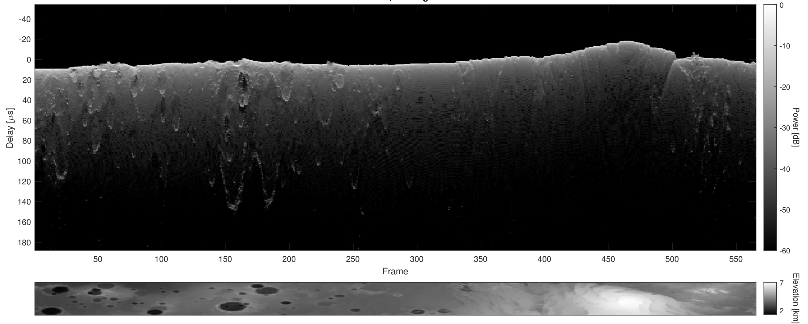
Orbit 4507, Cluttergram
