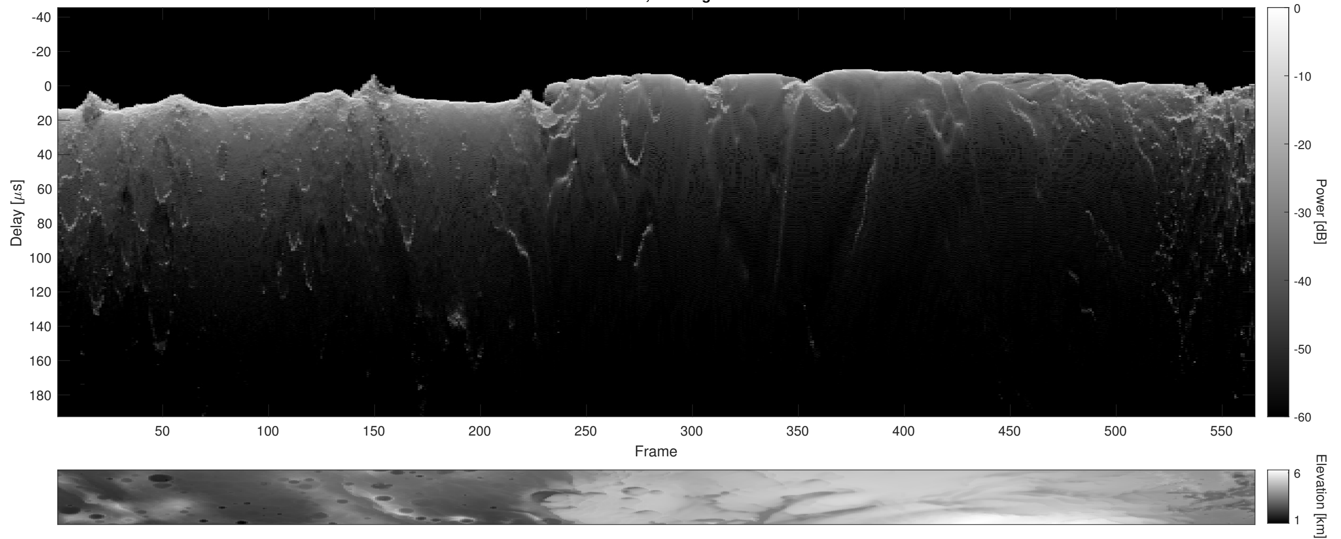
Orbit 4508, Cluttergram
