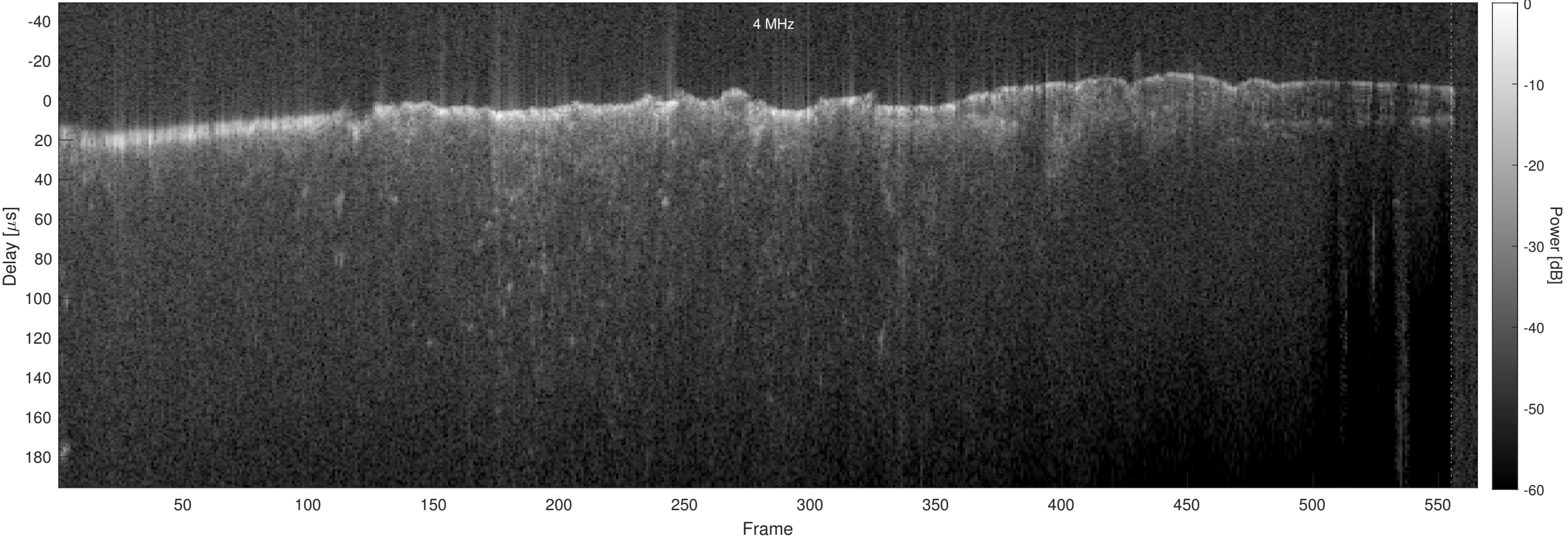
Orbit 4509, Optimized, No Window, Channel 2
