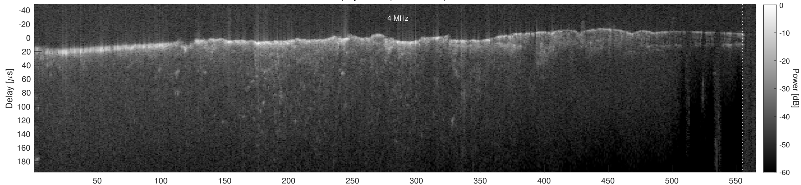
Orbit 4509, Cluttergram
