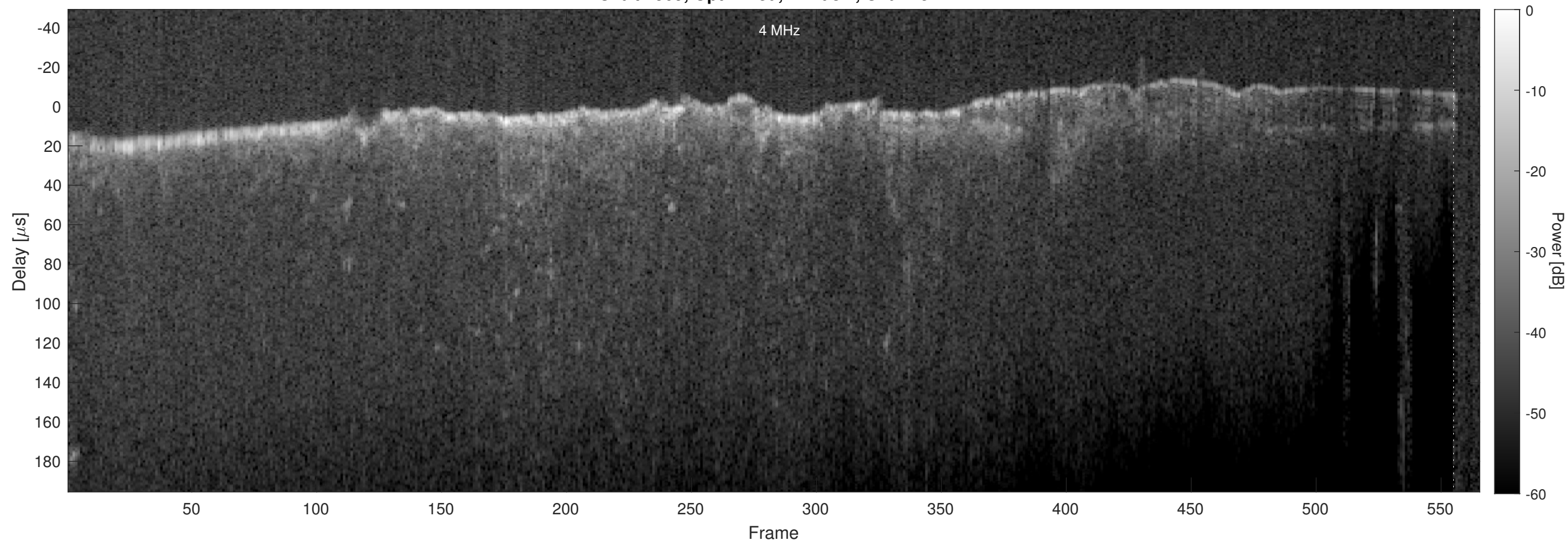
Orbit 4509, Optimized, Window, Channel 2
