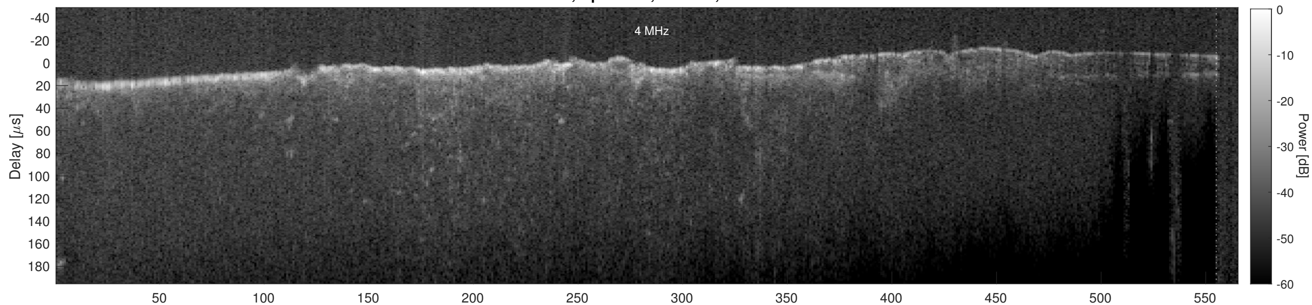
Orbit 4509, Cluttergram
