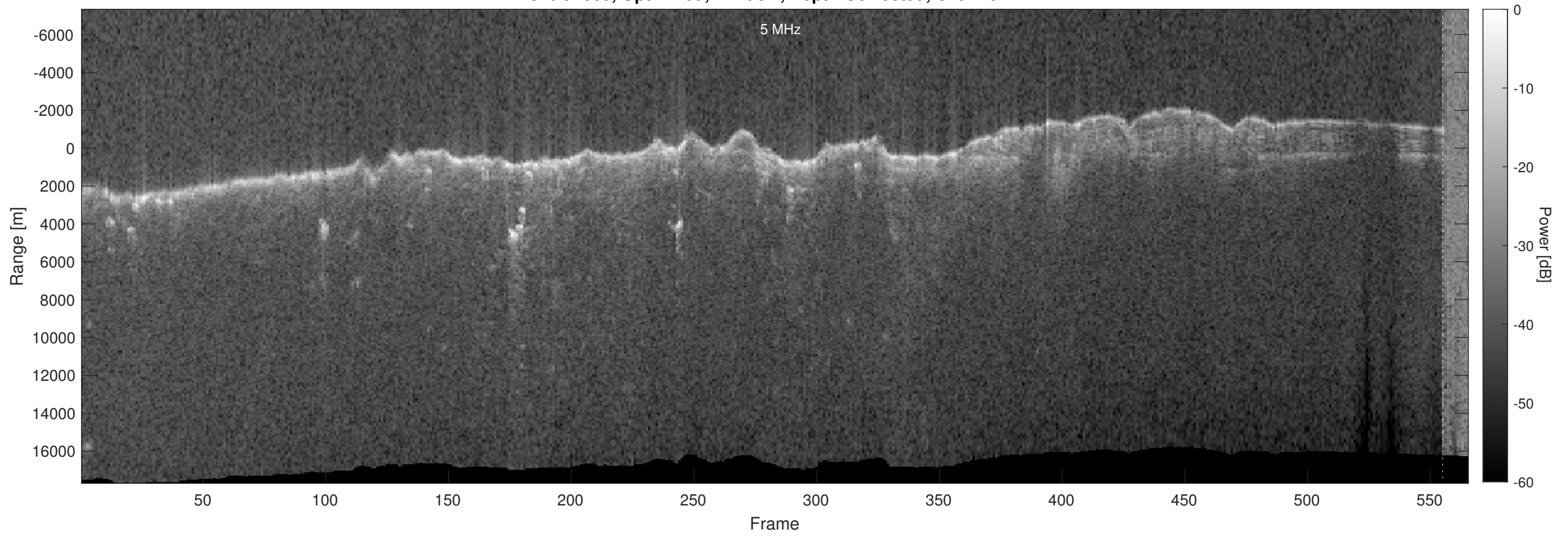
Orbit 4509, Optimized, Window, Depth-Corrected, Channel 2
