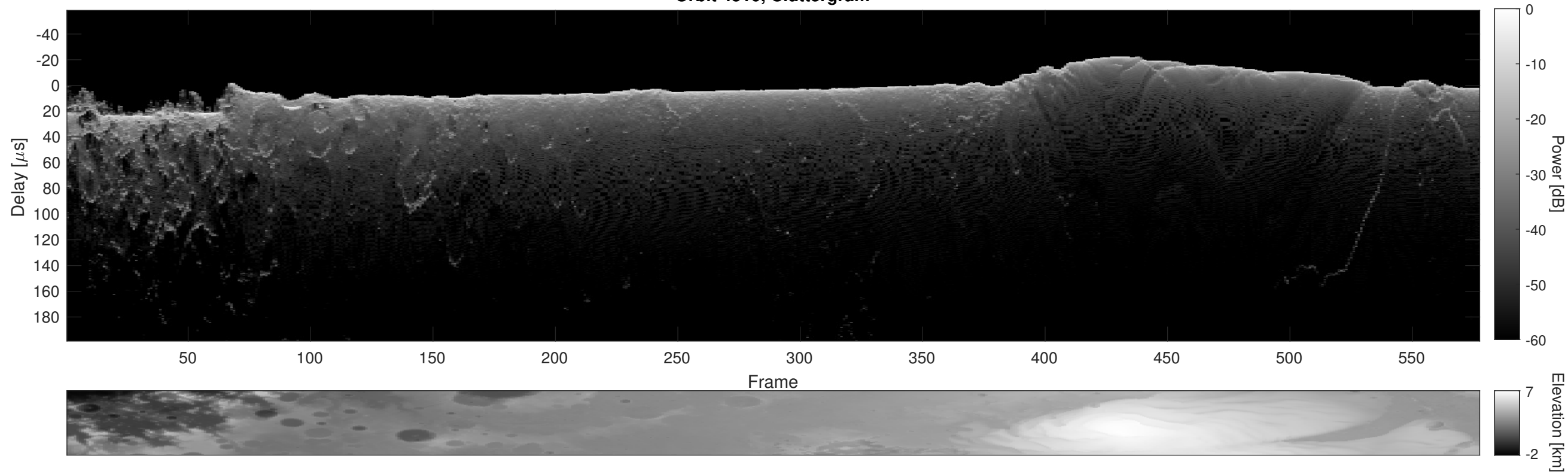
Orbit 4510, Cluttergram
