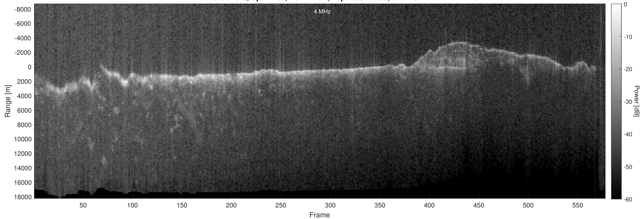
Orbit 4510, Optimized, No Window, Depth-Corrected, Channel 2
