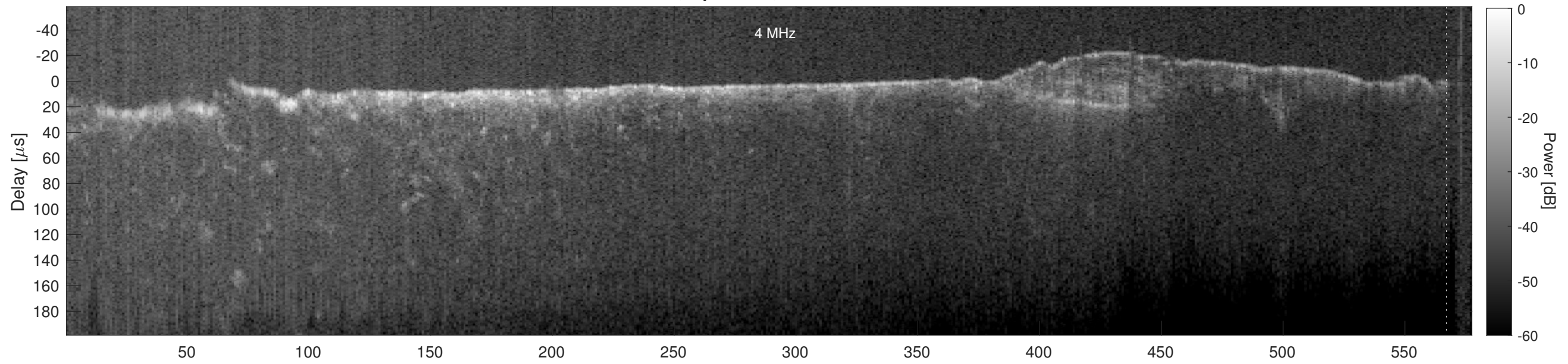
Orbit 4510, Cluttergram
