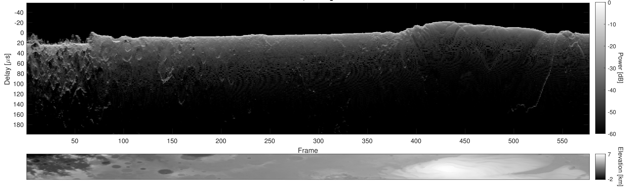
Orbit 4510, Cluttergram
