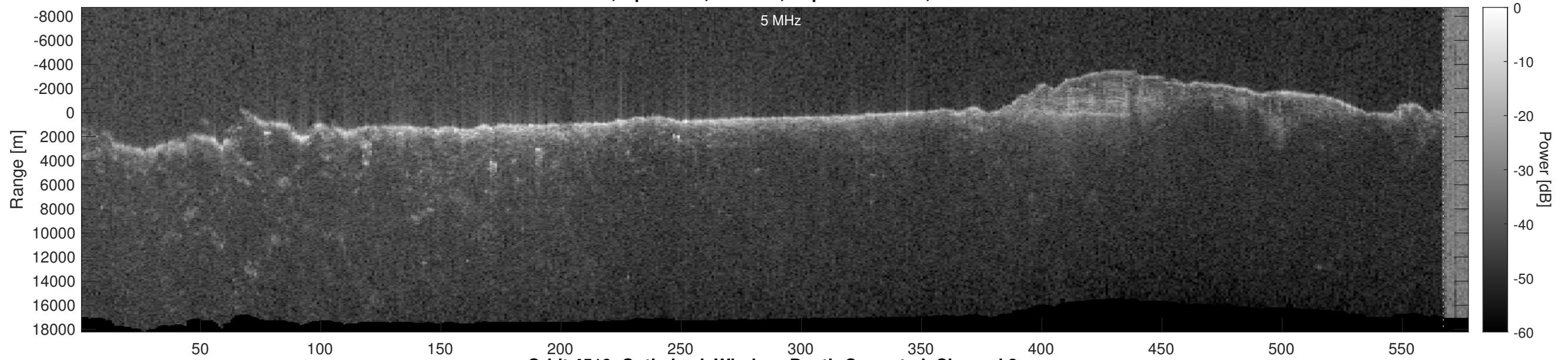
Orbit 4510, Optimized, Window, Depth-Corrected, Channel 2
