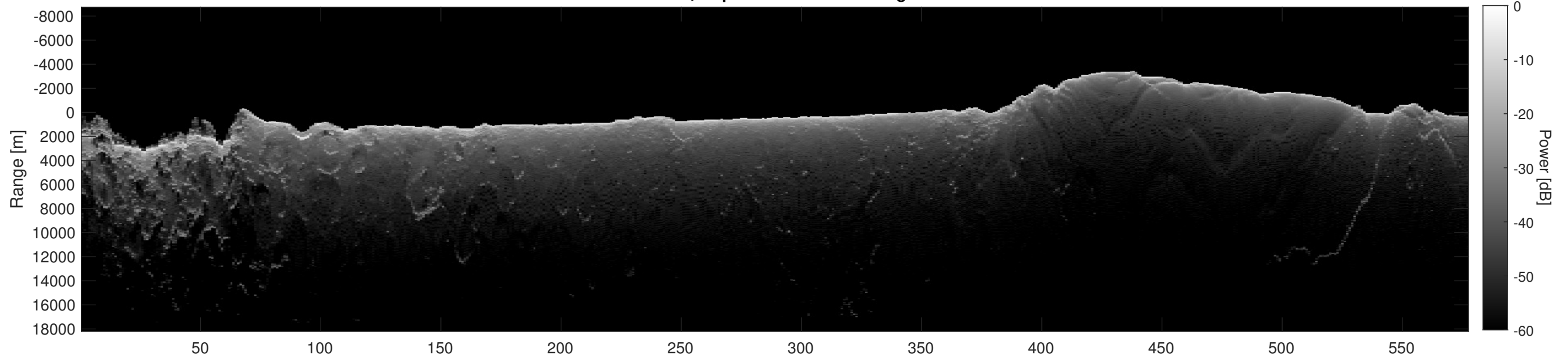
Orbit 4510, Depth-Corrected Cluttergram
