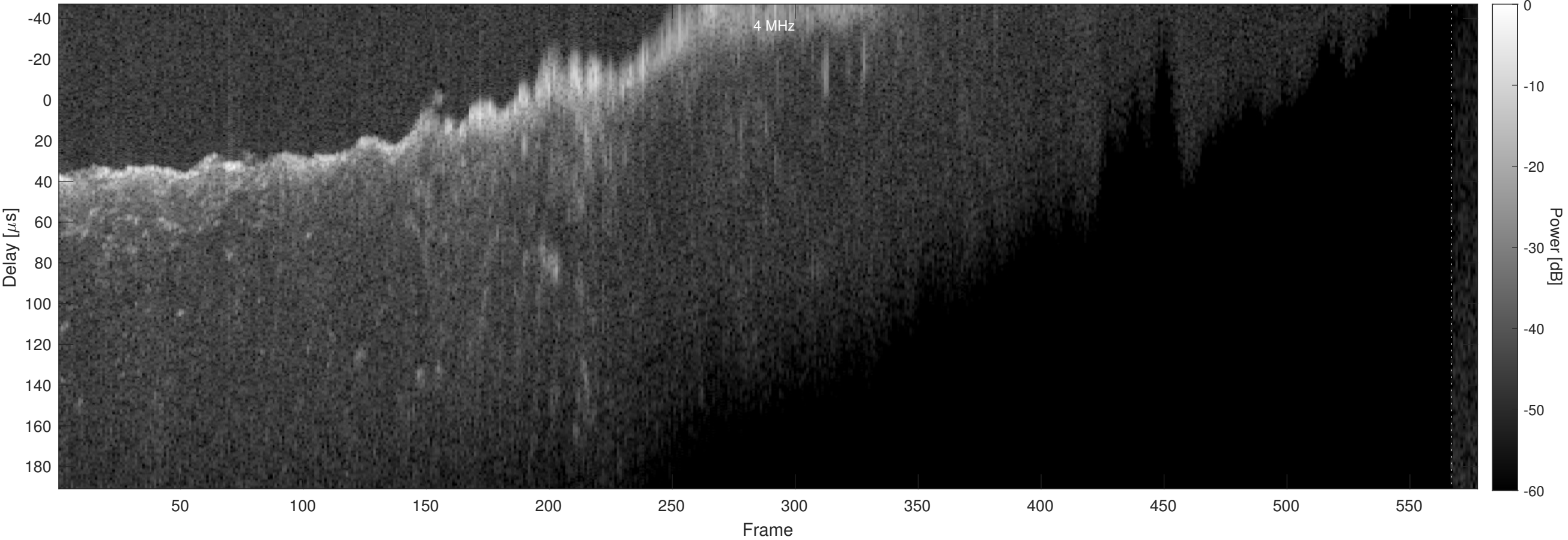
Orbit 4513, Chapman, Window, Channel 2
