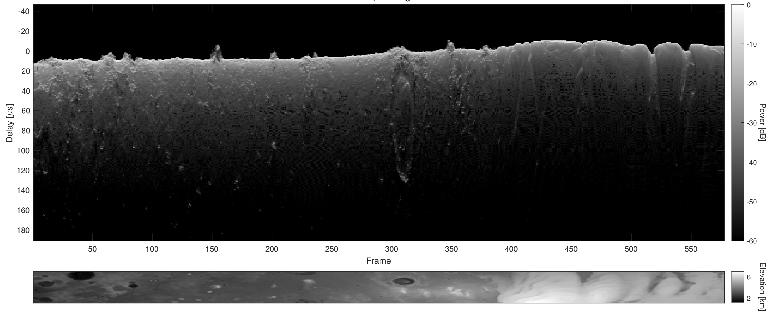
Orbit 4513, Cluttergram
