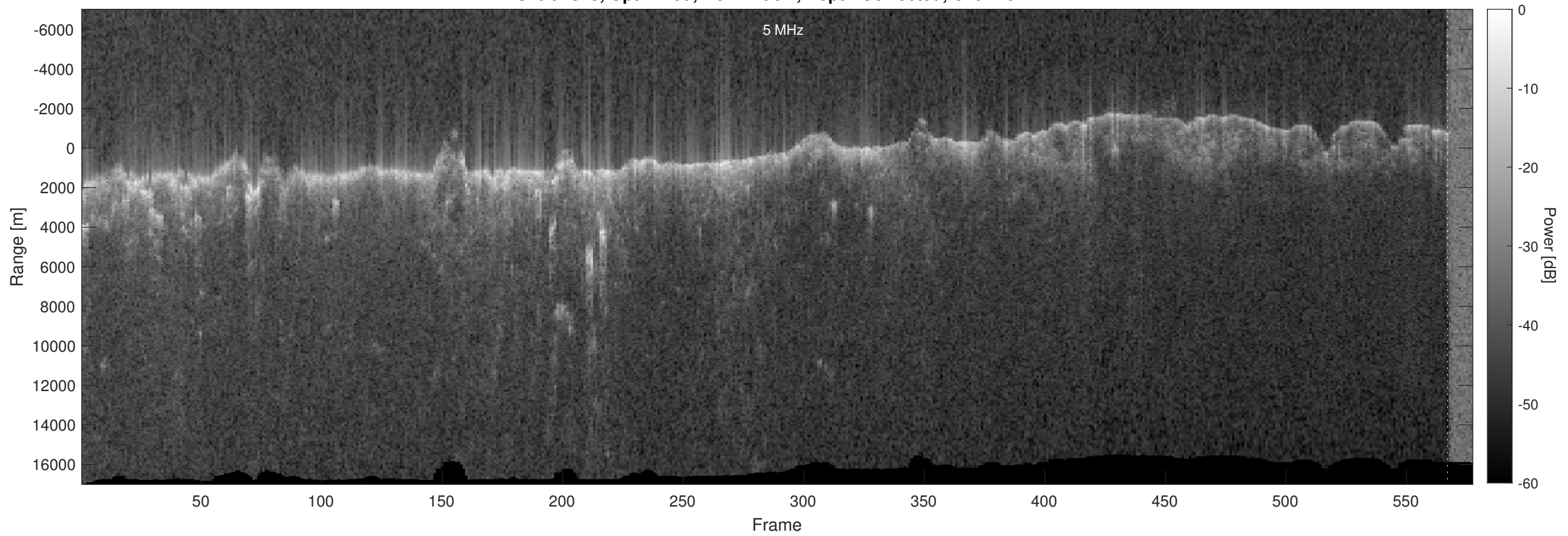
Orbit 4513, Optimized, No Window, Depth-Corrected, Channel 2
