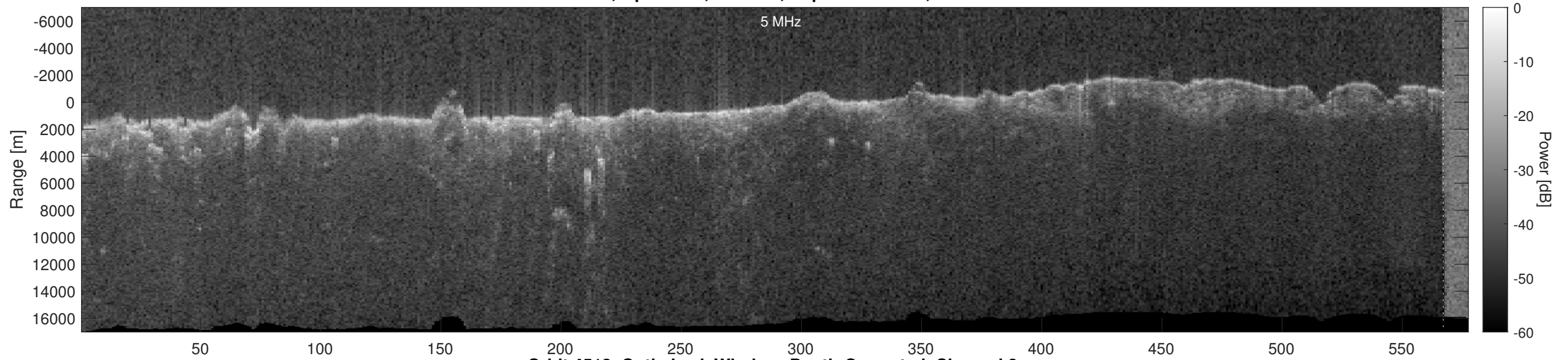
Orbit 4513, Optimized, Window, Depth-Corrected, Channel 2
