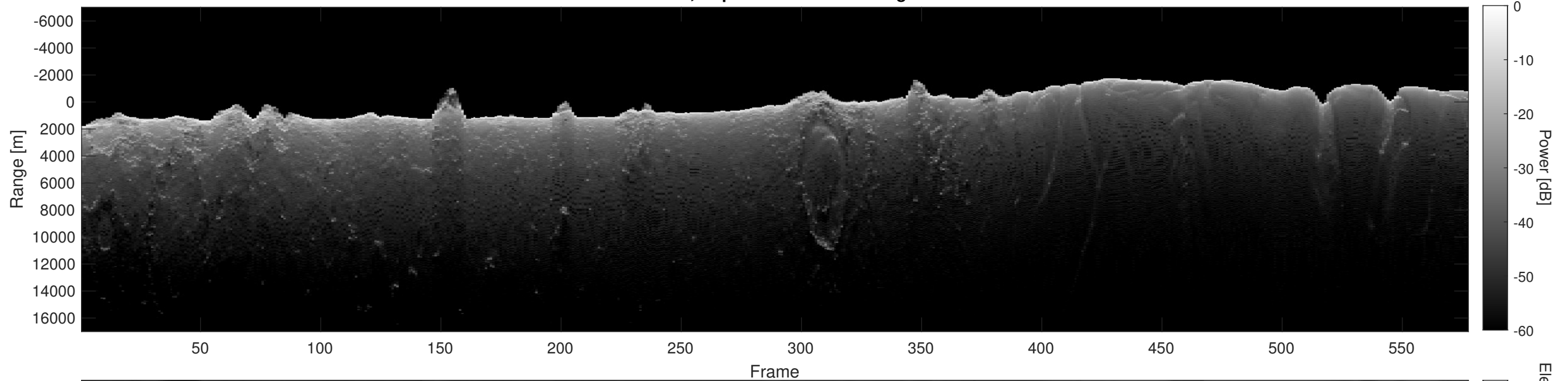
Orbit 4513, Depth-Corrected Cluttergram
