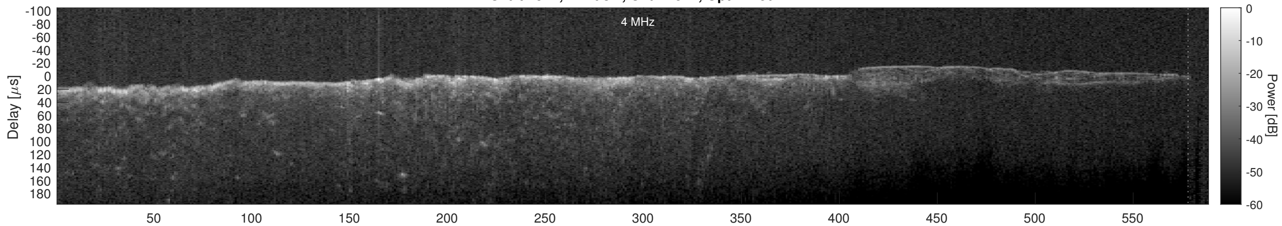
Orbit 4517, Cluttergram
