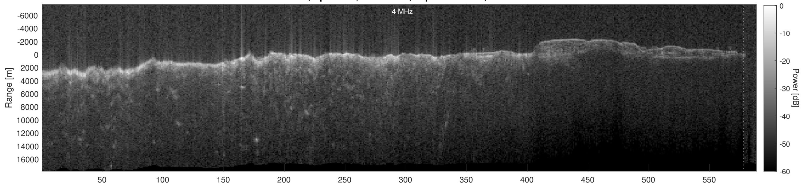
Orbit 4517, Depth-Corrected Cluttergram
