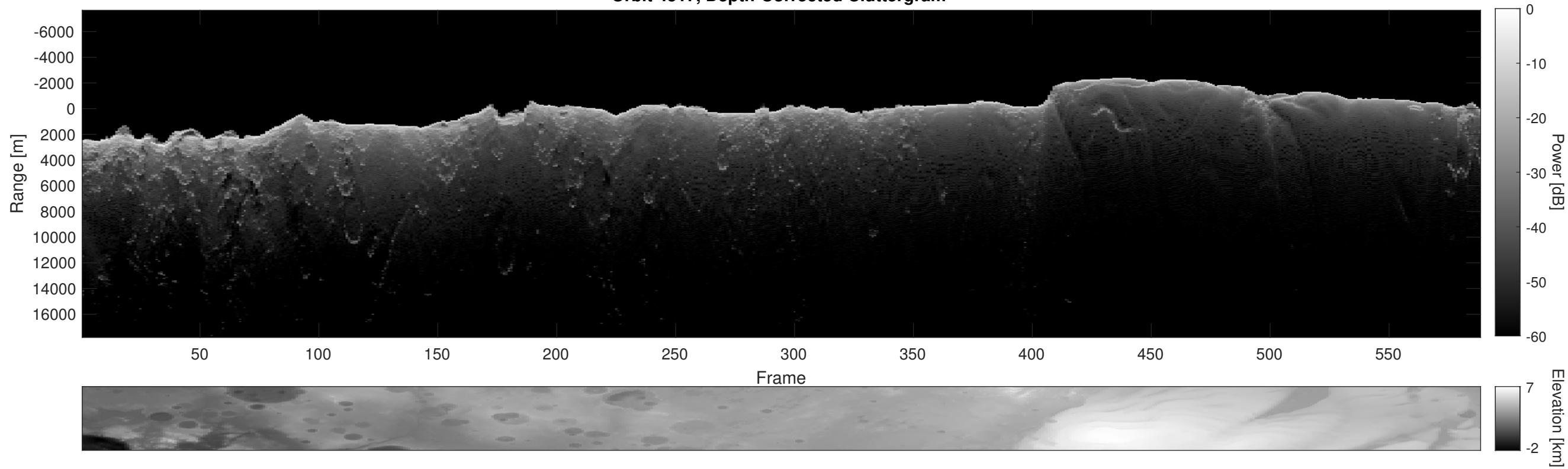
Orbit 4517, Depth-Corrected Cluttergram
