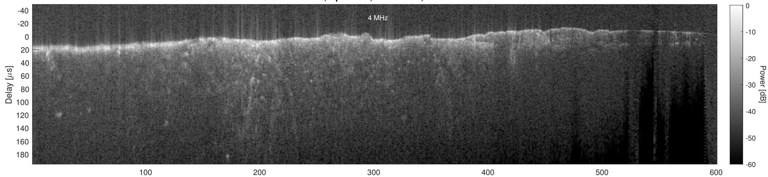
Orbit 4520, Cluttergram
