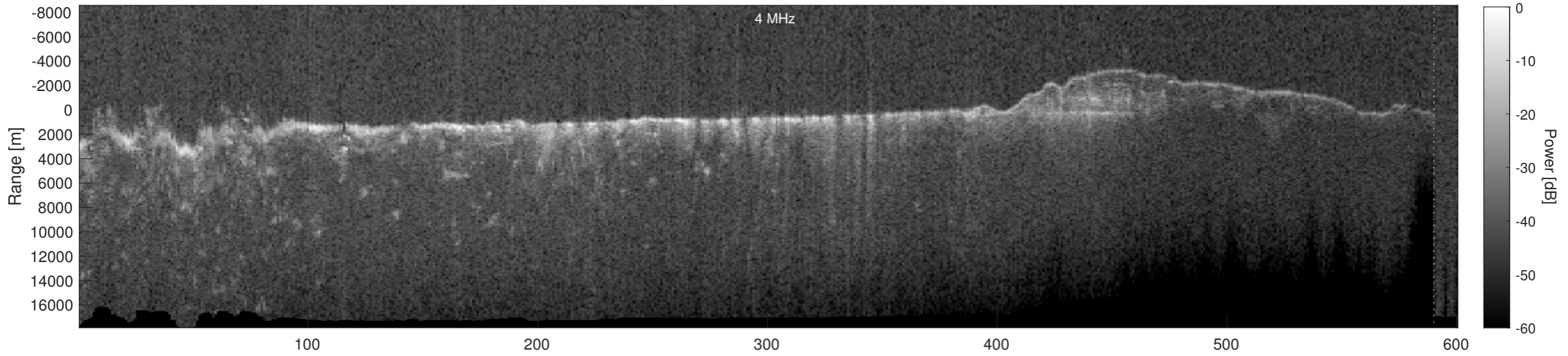
Orbit 4521, Depth-Corrected Cluttergram
