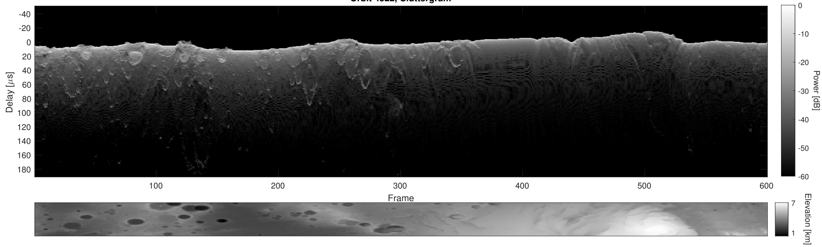
Orbit 4522, Cluttergram
