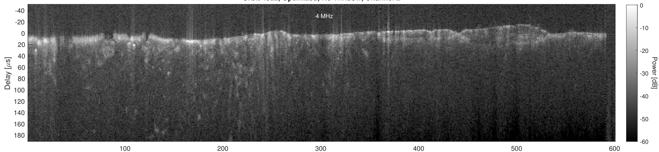
Orbit 4522, Cluttergram
