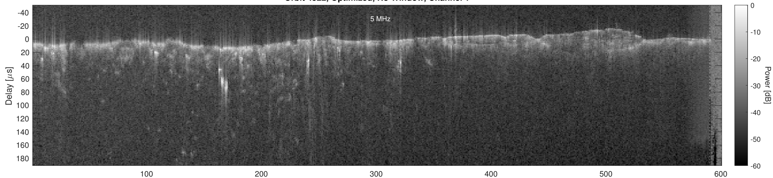
Orbit 4522, Optimized, No Window, Channel 2
