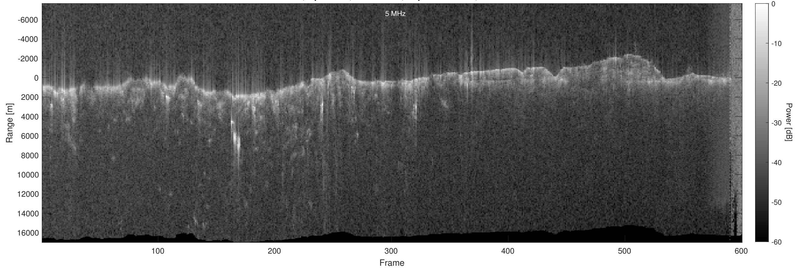
Orbit 4522, Optimized, No Window, Depth-Corrected, Channel 2
