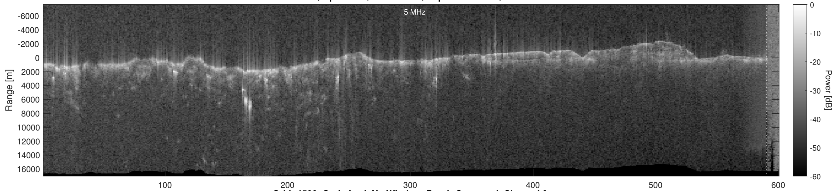
Orbit 4522, Optimized, No Window, Depth-Corrected, Channel 2
