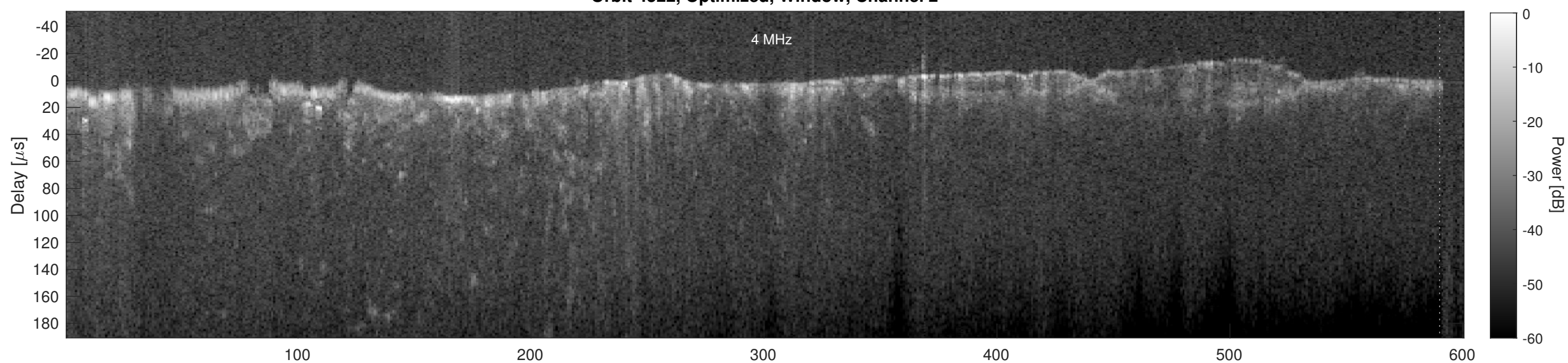
Orbit 4522, Cluttergram
