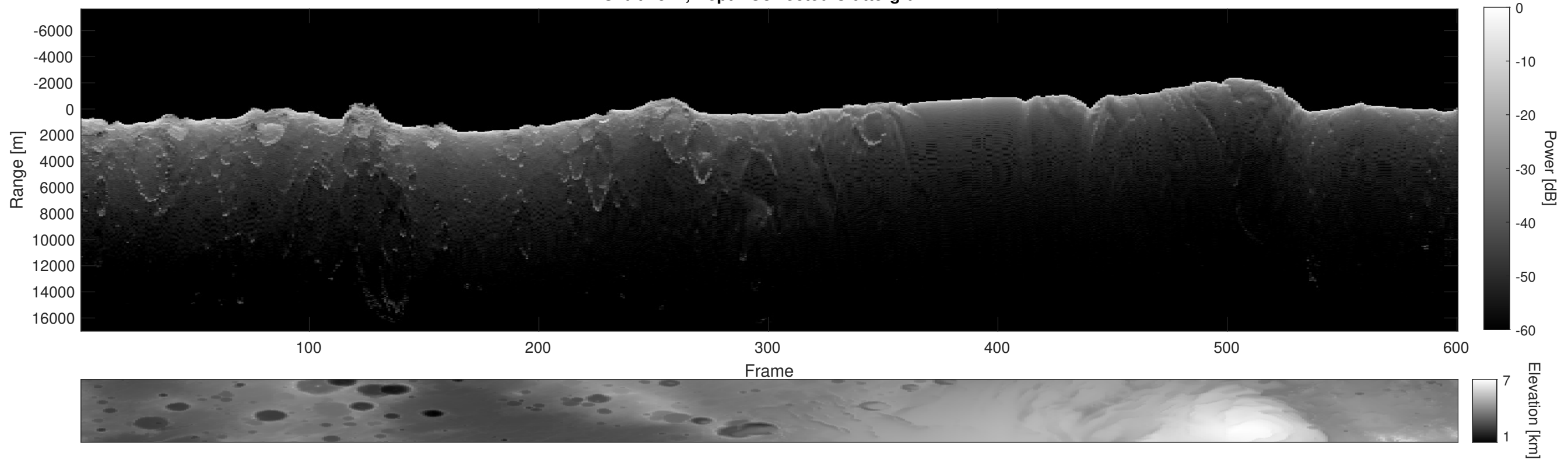
Orbit 4522, Depth-Corrected Cluttergram
