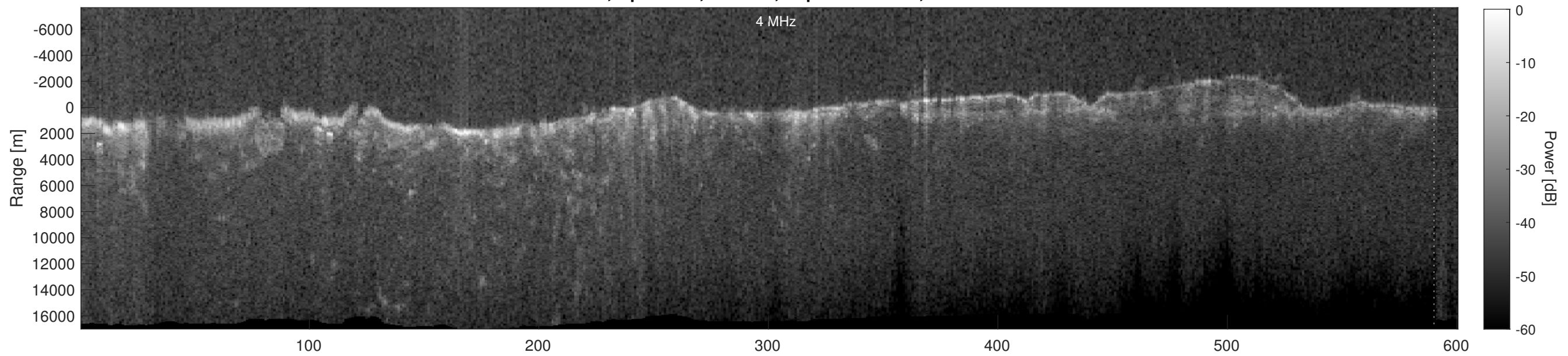
Orbit 4522, Depth-Corrected Cluttergram
