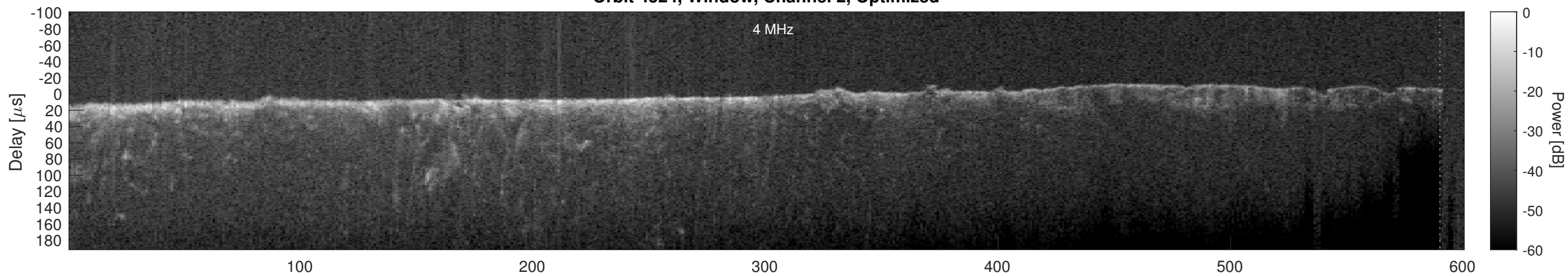
Orbit 4524, Cluttergram
