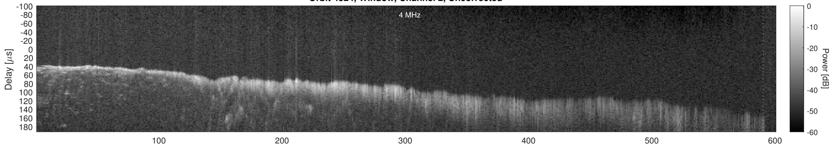
Orbit 4524, Window, Channel 2, Chapman
