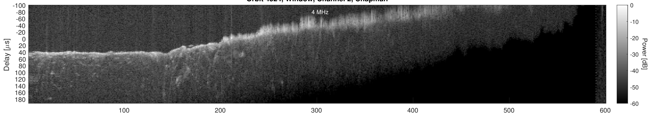
Orbit 4524, Window, Channel 2, Optimized
