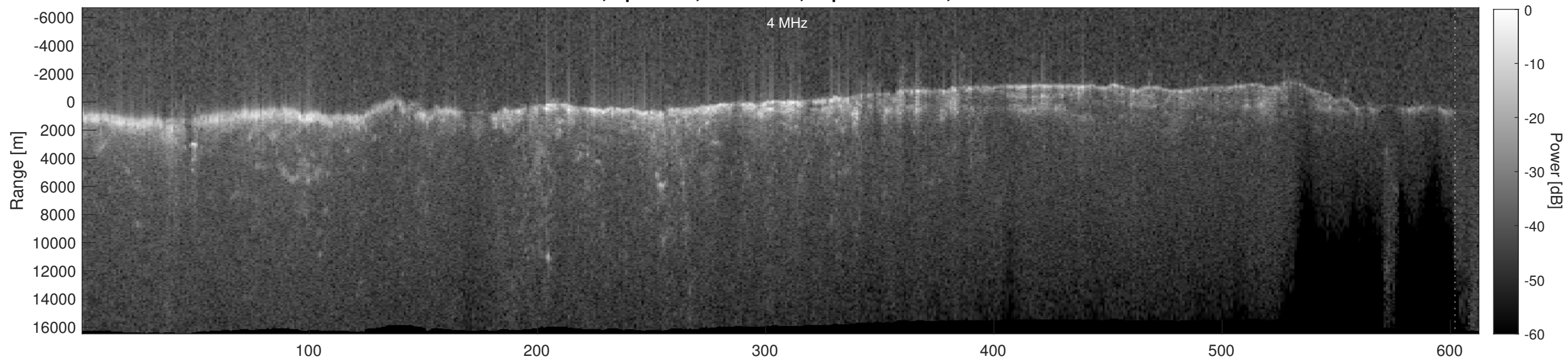
Orbit 4526, Depth-Corrected Cluttergram
