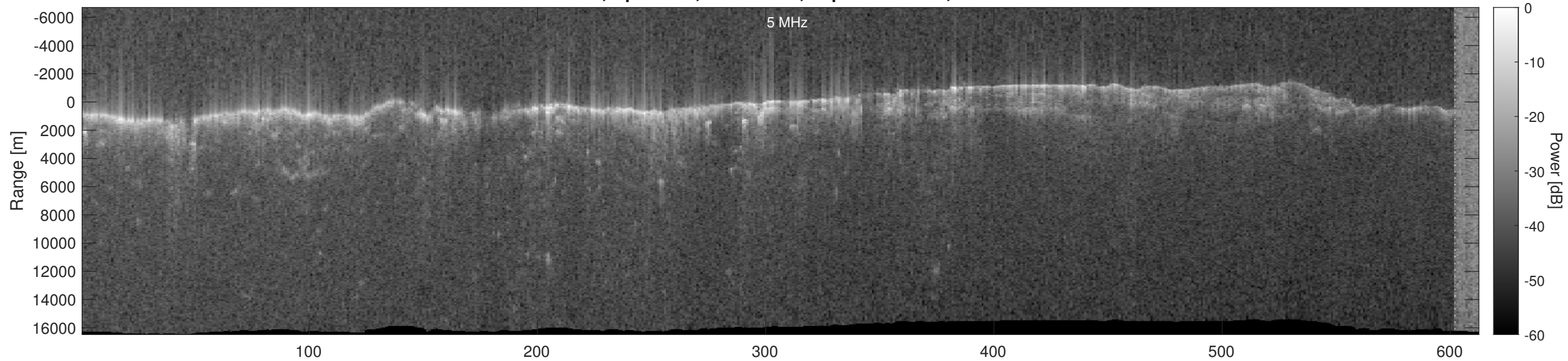
Orbit 4526, Optimized, No Window, Depth-Corrected, Channel 2
