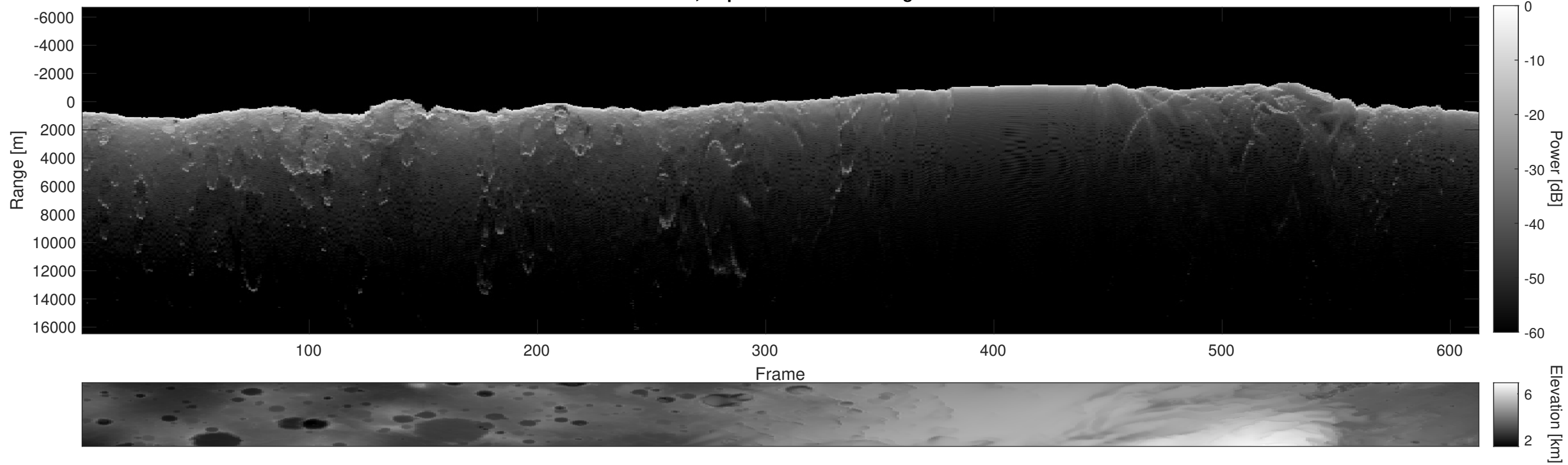
Orbit 4526, Depth-Corrected Cluttergram
