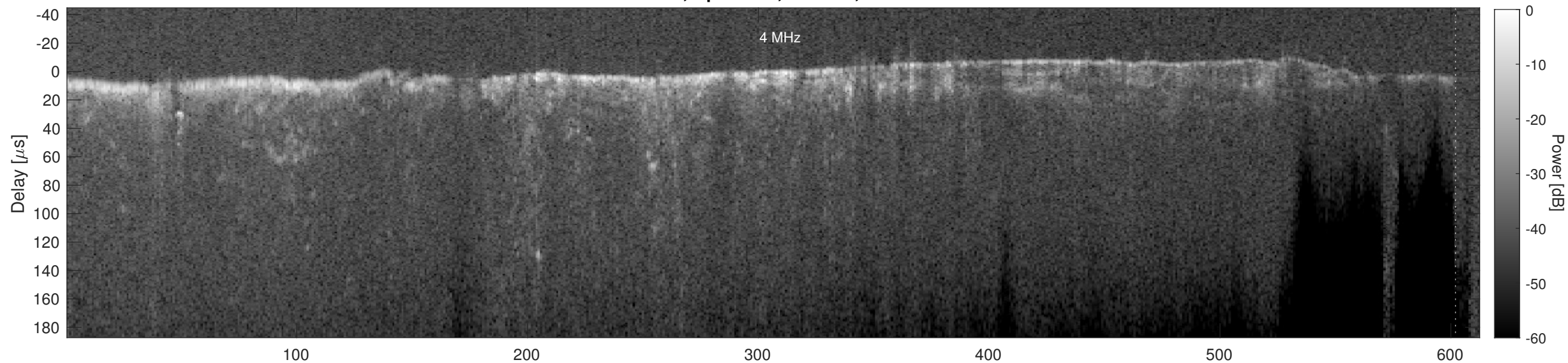
Orbit 4526, Cluttergram
