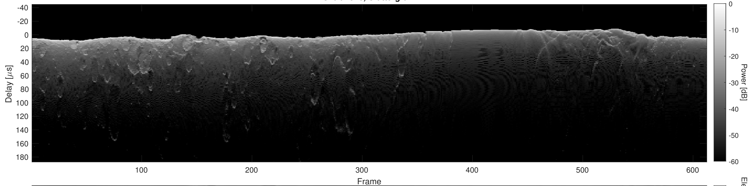
Orbit 4526, Cluttergram
