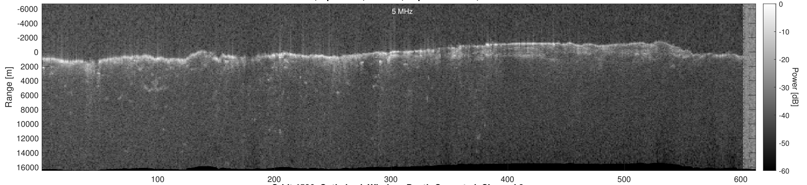
Orbit 4526, Optimized, Window, Depth-Corrected, Channel 2
