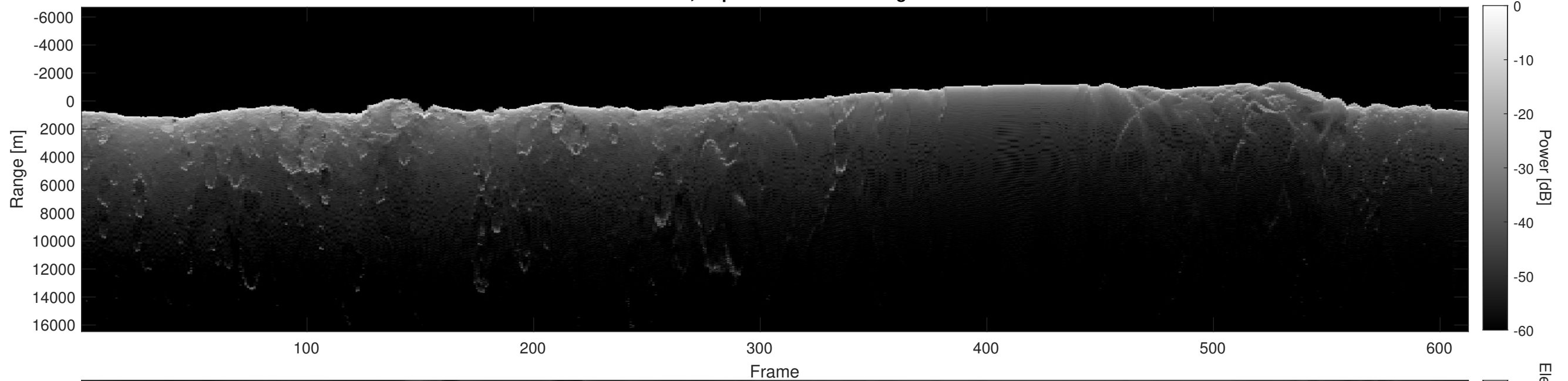
Orbit 4526, Depth-Corrected Cluttergram
