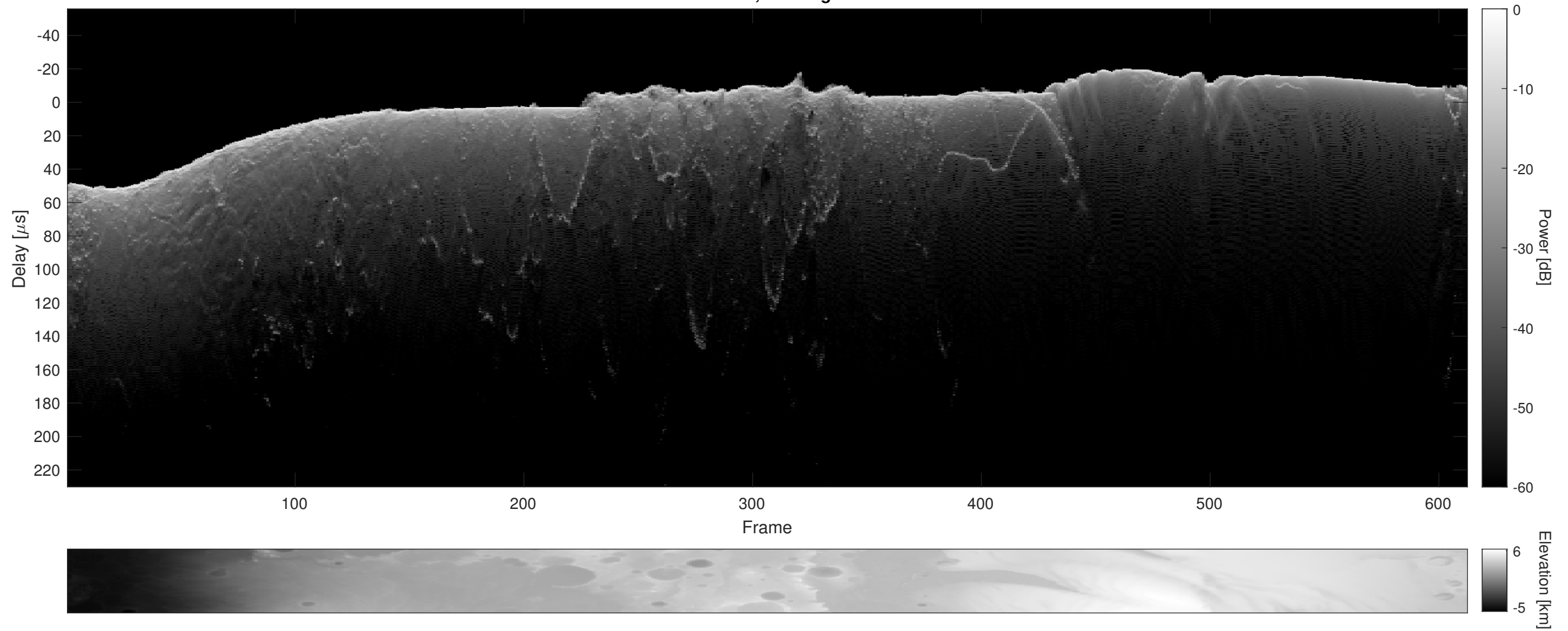
Orbit 4527, Cluttergram
