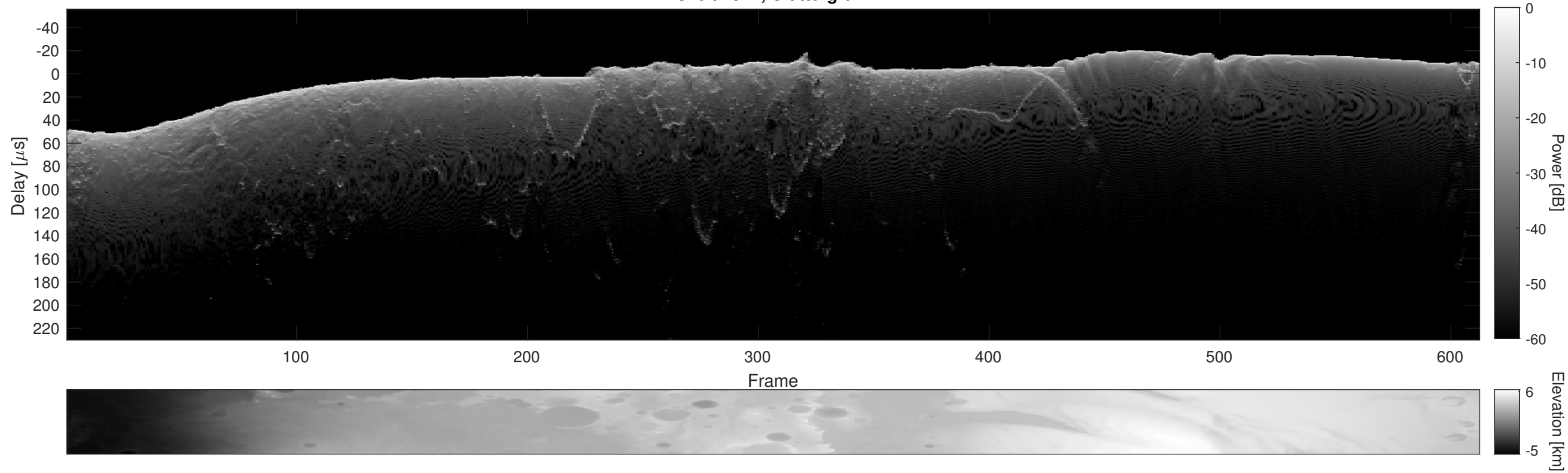
Orbit 4527, Cluttergram
