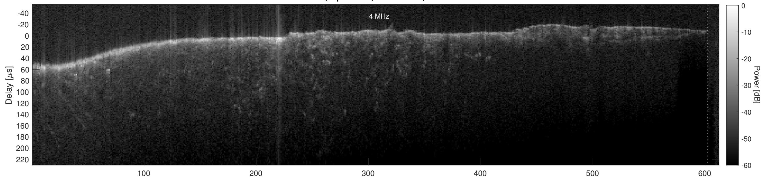
Orbit 4527, Cluttergram
