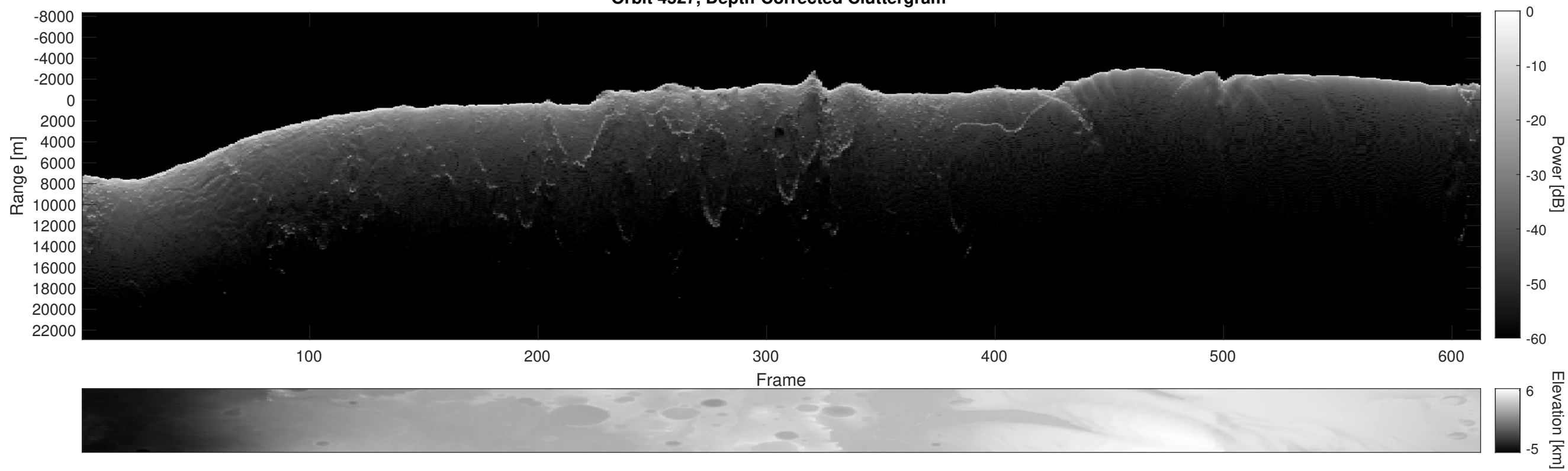
Orbit 4527, Depth-Corrected Cluttergram
