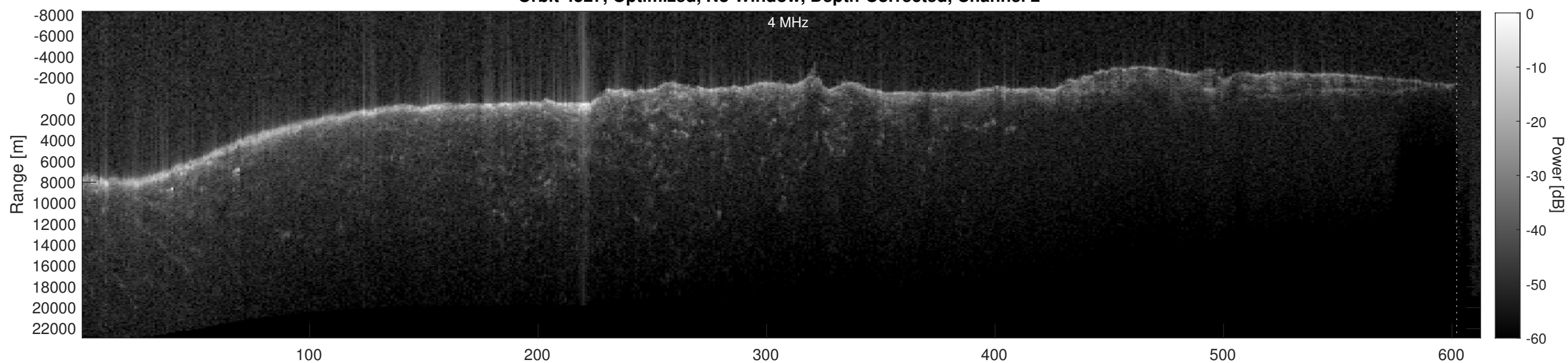
Orbit 4527, Depth-Corrected Cluttergram
