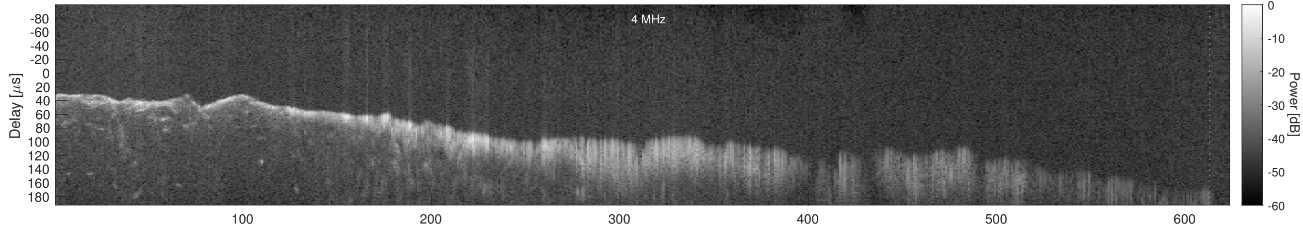
Orbit 4530, Window, Channel 2, Chapman
