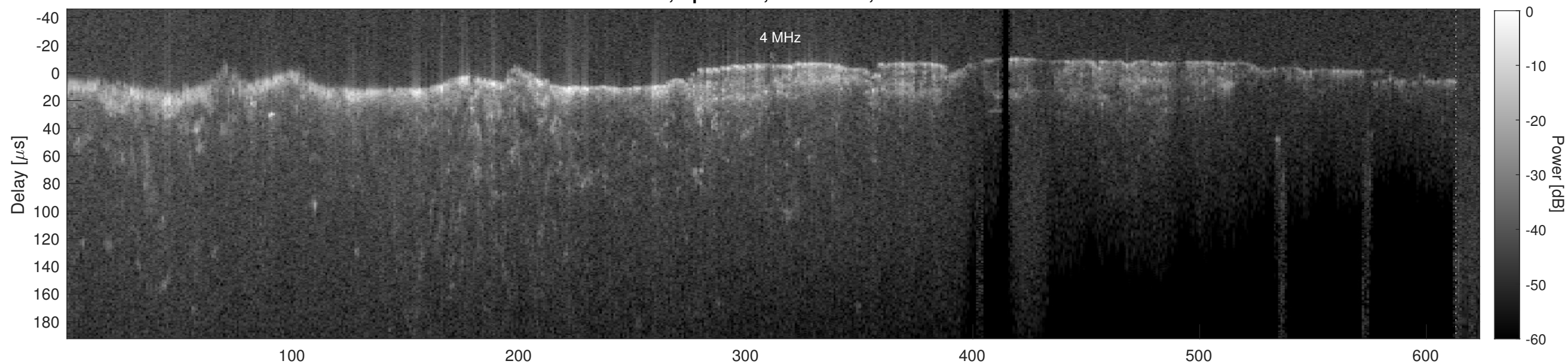
Orbit 4530, Cluttergram
