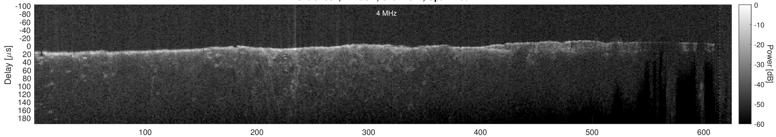
Orbit 4531, Cluttergram
