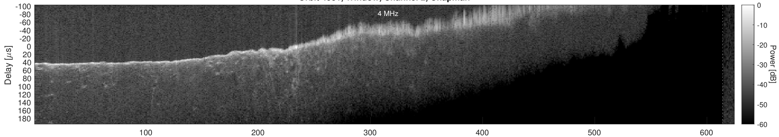
Orbit 4531, Window, Channel 2, Optimized
