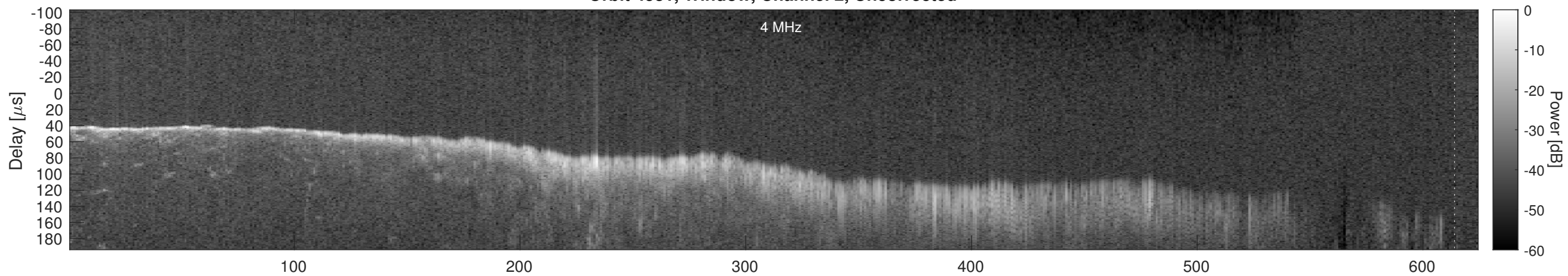
Orbit 4531, Window, Channel 2, Chapman
