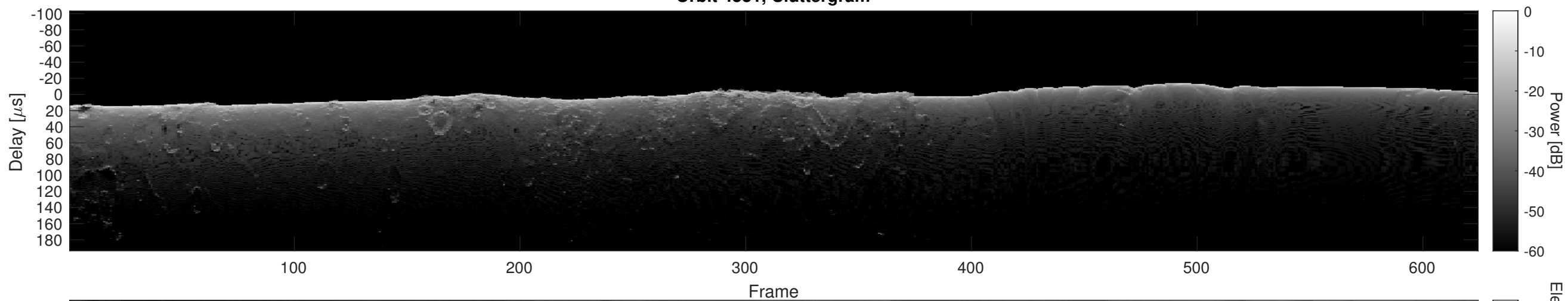
Orbit 4531, Cluttergram
