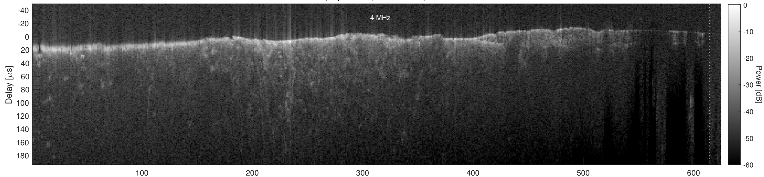
Orbit 4531, Cluttergram
