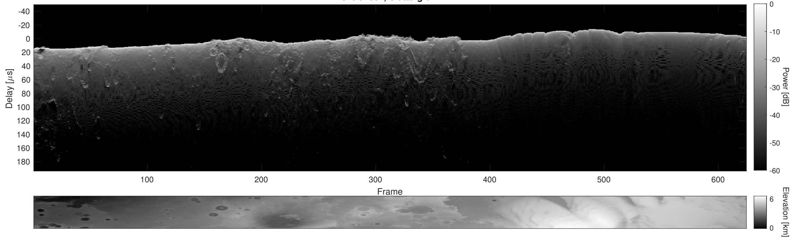
Orbit 4531, Cluttergram
