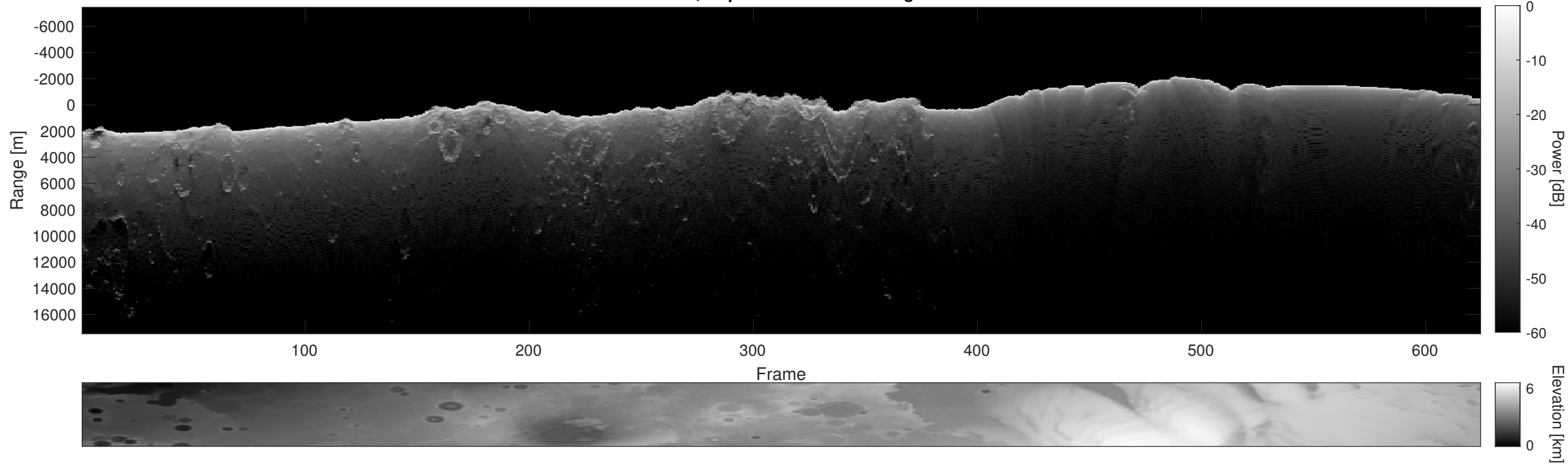
Orbit 4531, Depth-Corrected Cluttergram
