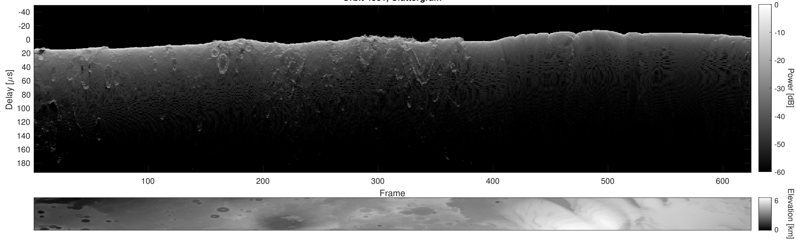
Orbit 4531, Cluttergram
