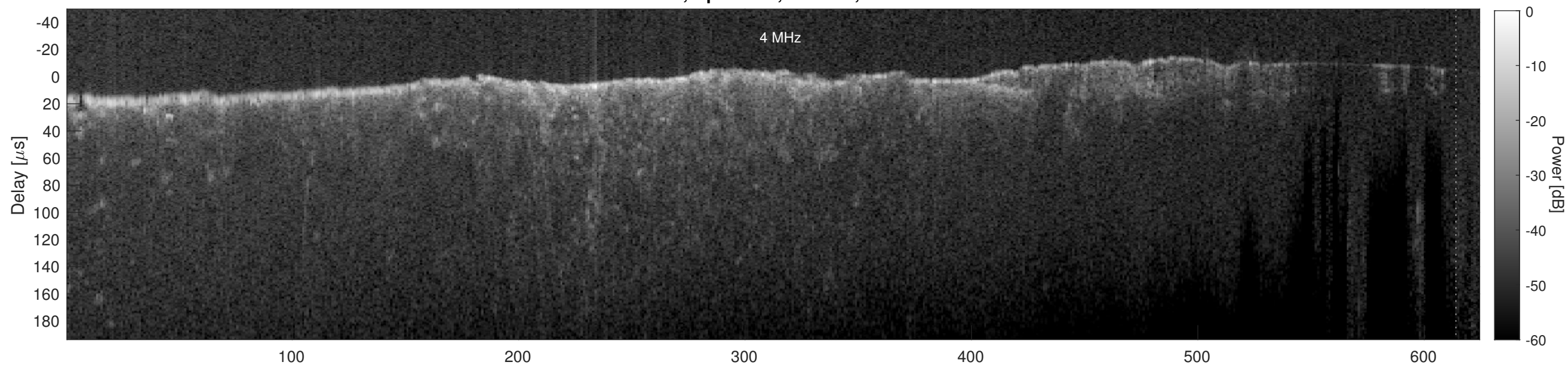
Orbit 4531, Cluttergram
