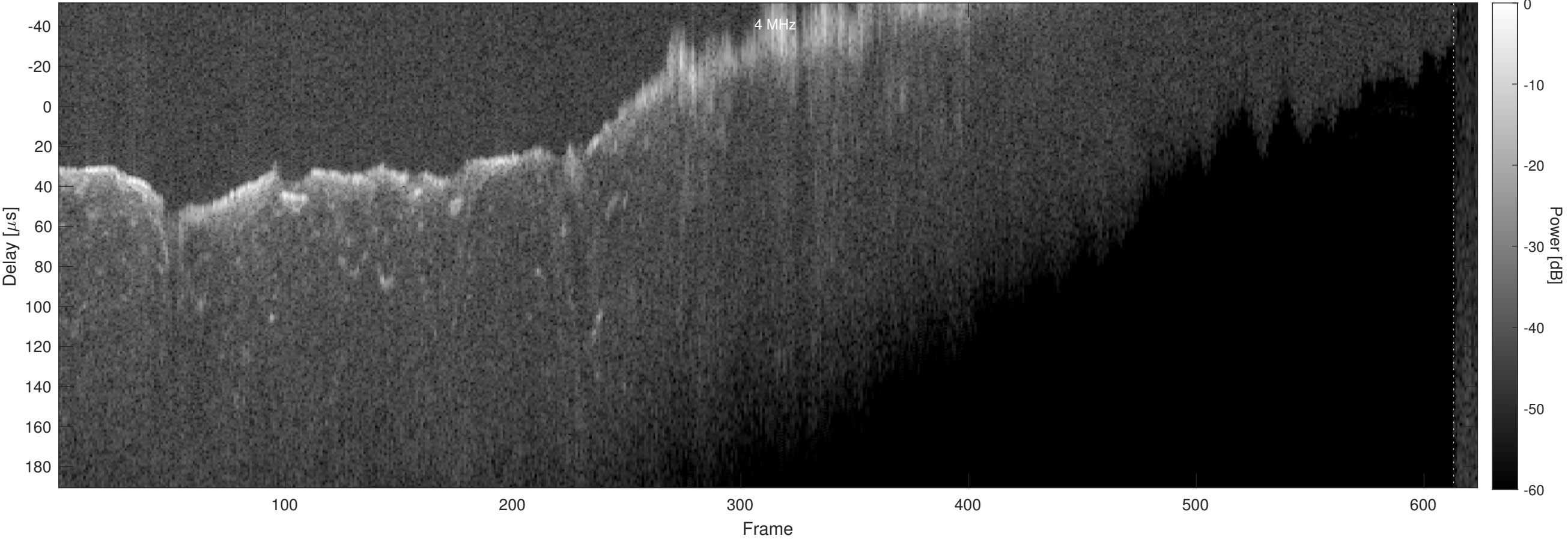
Orbit 4533, Chapman, Window, Channel 2
