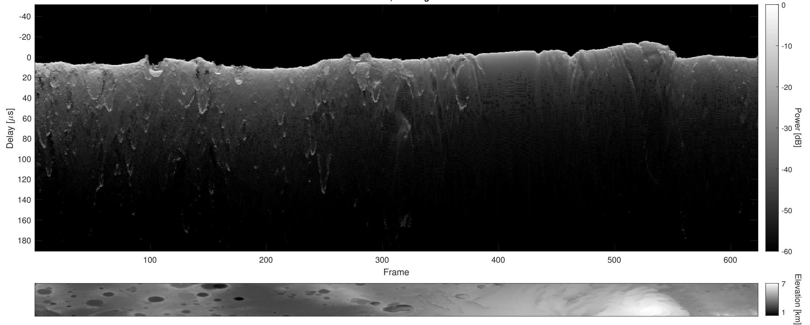
Orbit 4533, Cluttergram
