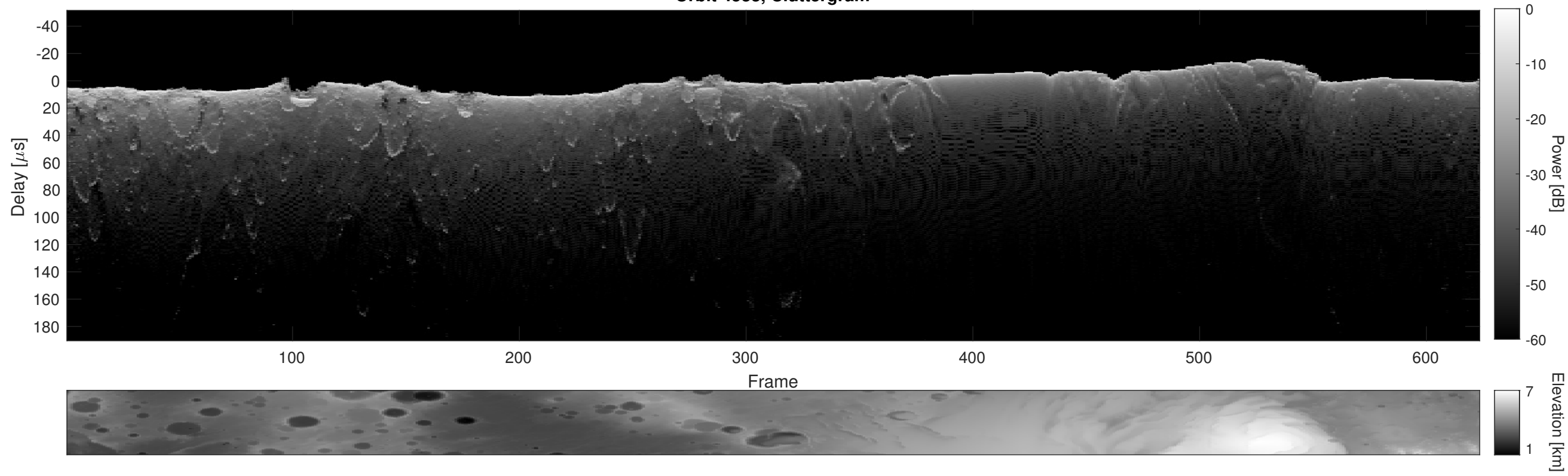
Orbit 4533, Cluttergram
