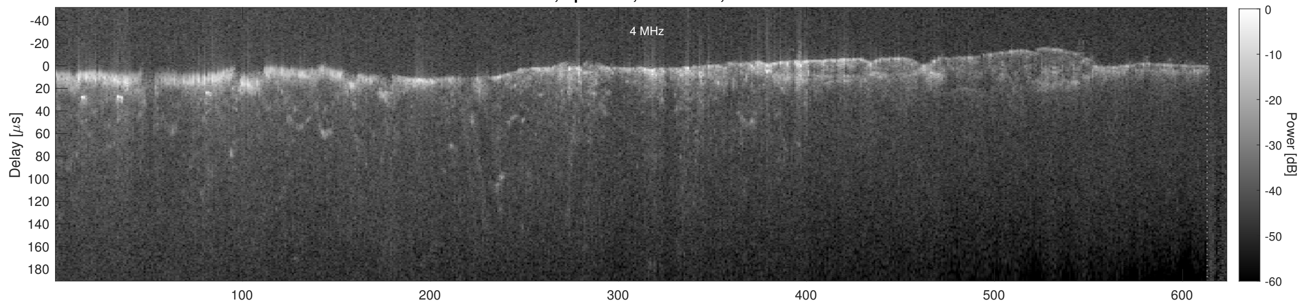
Orbit 4533, Cluttergram
