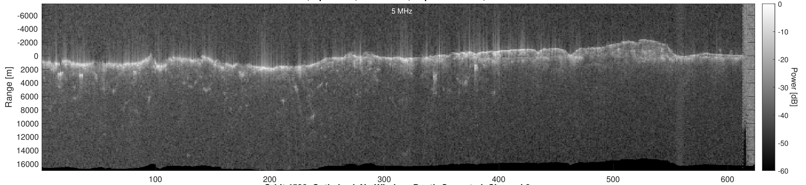
Orbit 4533, Optimized, No Window, Depth-Corrected, Channel 2
