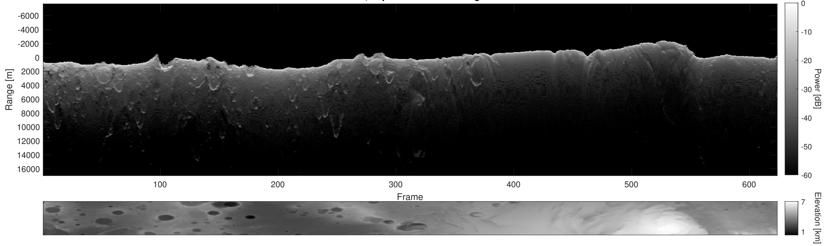
Orbit 4533, Depth-Corrected Cluttergram
