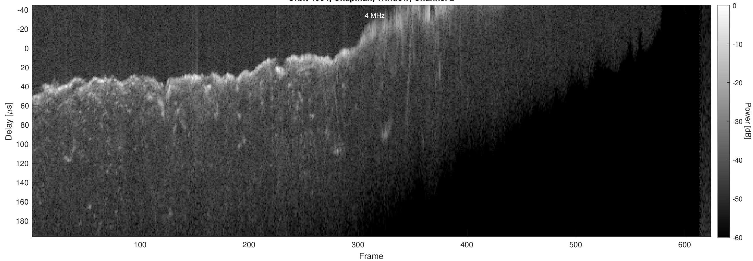
Orbit 4534, Chapman, Window, Channel 2
