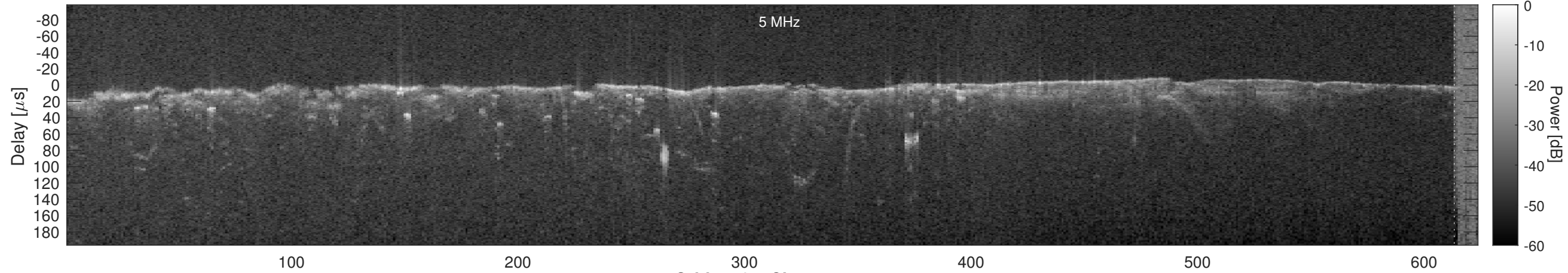
Orbit 4534, Cluttergram
