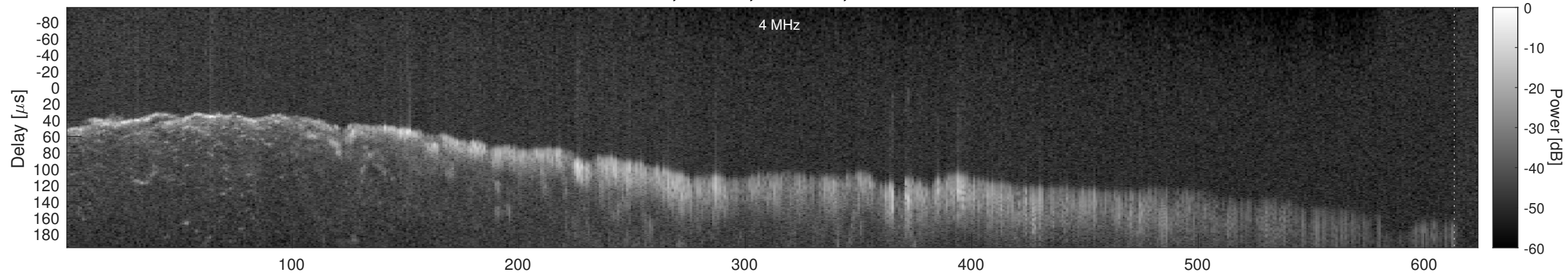
Orbit 4534, Window, Channel 2, Chapman
