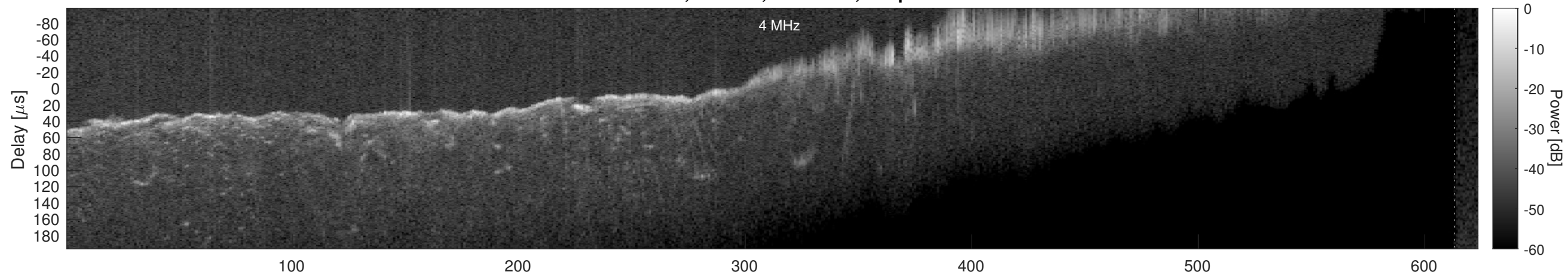
Orbit 4534, Window, Channel 2, Optimized
